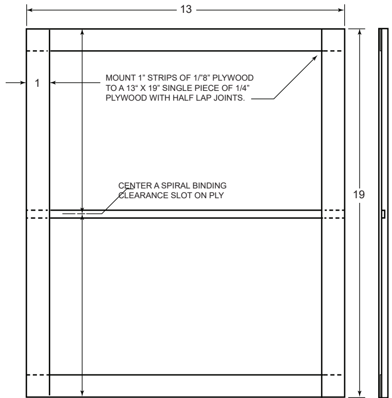
BASE
